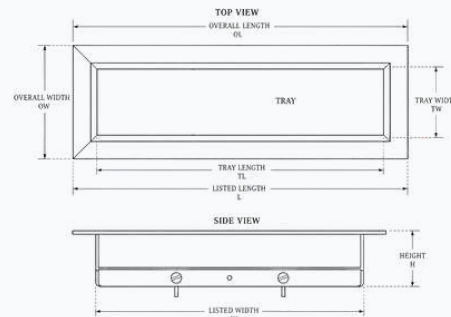
DIMENSION CHART
