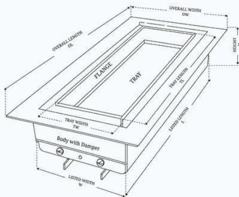
DIMENSION CHART
