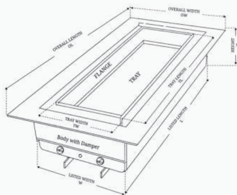
DIMENSION CHART
