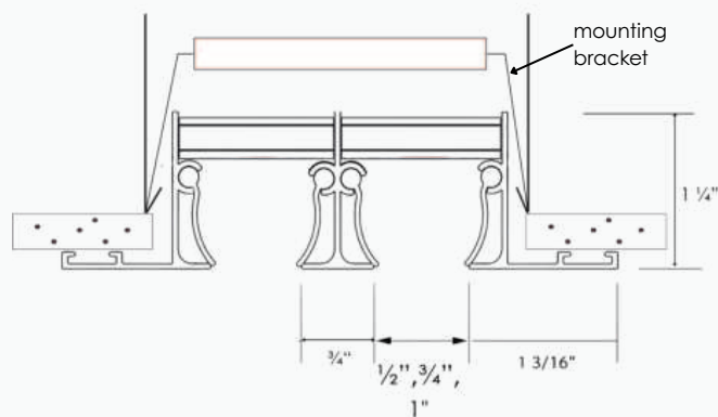
DIFFUSER WITH PATTERN CONTROL
