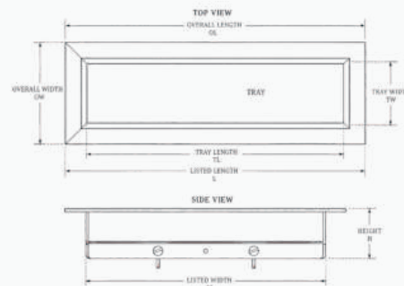
DIMENSION CHART
