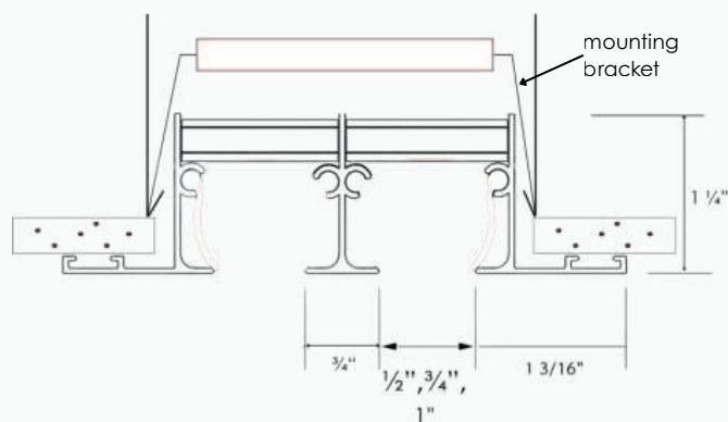
DIFFUSER ONLY
